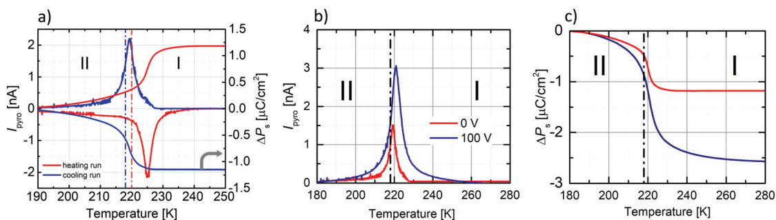
Fig. 8 (a) The left Y-scale presents the temperature dependencies of I_{\text{pyro}} measured on unpoled crystal along the c-axis upon cooling and heating runs, while the right Y-scale the temperature dependence of \Delta P_s . Dash-dot lines indicate the onset temperature based on DSC curves (blue-cooling run at 218 K, red-heating cycle at 220 K). (b) Temperature dependence of I_{\text{pyro}} measured on unpoled ( 0 \text{ kV cm}^{-1} ) sample and after an application of the external electric field ( \pm 1.32 \text{ kV cm}^{-1} ) in phase II and then heating the sample to phase I. The measurements of I_{\text{pyro}} were carried out during cooling. (c) \Delta P_s(T) as calculated from the I_{\text{pyro}} data.
