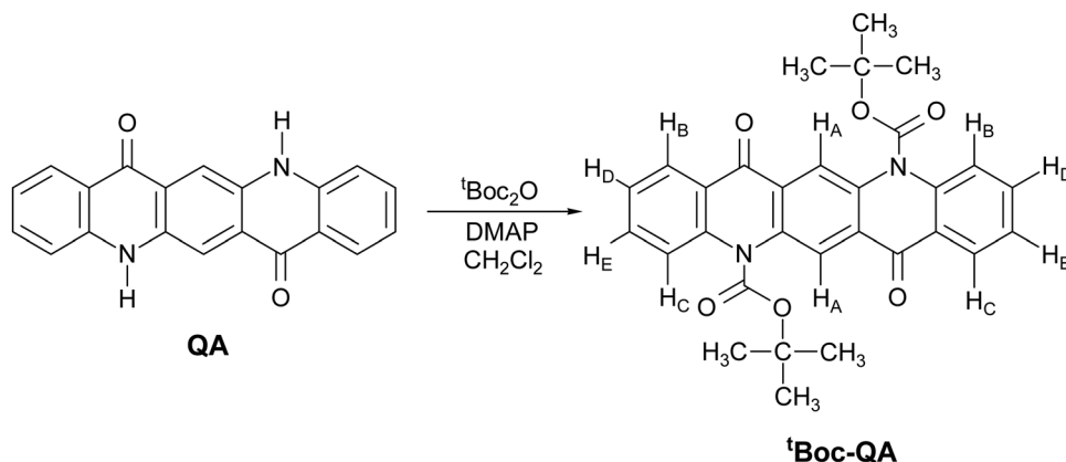
Fig. 1 Synthetic route from quinacridone pigment (QA) to the latent pigment ( t\text{Boc-QA} ).
