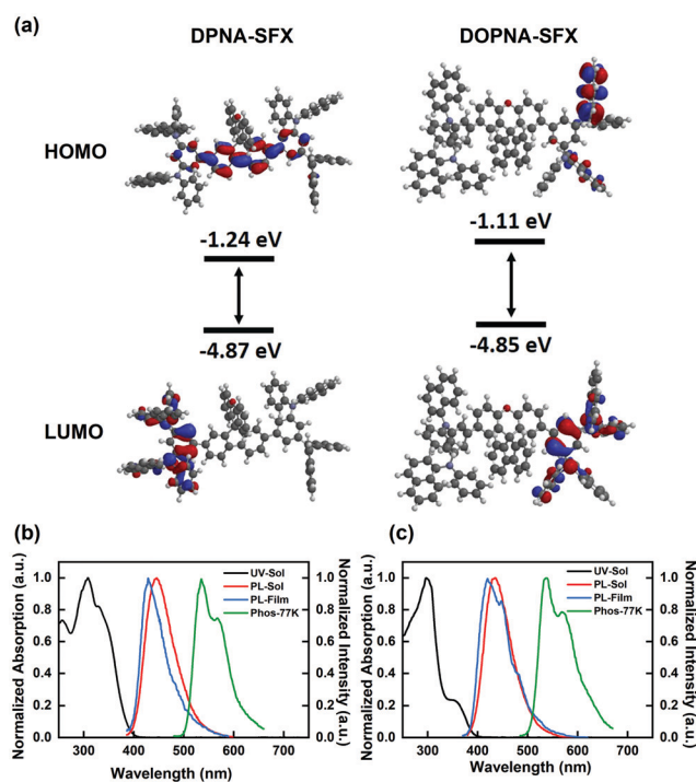
Fig. 1 (a) HOMO and LUMO distributions of DPNA-SFX and DOPNA-SFX; (b and c) UV-Vis absorption (in DCM solution), PL spectra (in DCM solution and in film at room temperature, in DCM solution at 77 K) of (b) DPNA-SFX; and (c) DOPNA-SFX.
