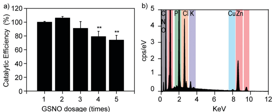
Fig. 6 (a) Catalytic efficiencies of 20% \text{Cu}^{2+} /ZIF-8 particles ( 0.1 \text{ mg mL}^{-1} ) after continuous addition of GSNO solutions ( 50 \text{ }\mu\text{M} ). Values represent mean \pm standard deviation, n = 3 . Statistical significance relative to the first dosage was calculated, **p < 0.01 (one-way ANOVA followed by Tukey post hoc test). (b) EDS spectrum of 20% \text{Cu}^{2+} /ZIF-8 after reaction with GSNO.
