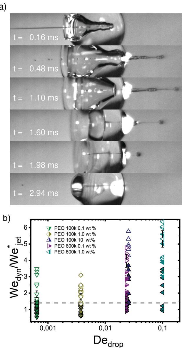
Fig. 7 (a) Snapshots of a liquid jet impacting a water droplet with PEO 600k 1 wt% showing pearling (see Movie S5 in the ESI†). A jet with U_{\text{jet}} = 33.5 m s -1 and We_{\text{jet}} = 1160 impacts a droplet with D_{\text{drop}} = 2.21 mm. The jet travels a distance larger than D_{\text{drop}} , but due to the viscoelastic effects of the droplet, it gets sucked back into the droplet. (b) Phase diagram in terms of De and We_{\text{dyn}}^*/We_{\text{jet}}^* . Open symbols represent cases where the jet traverses the droplet, solid ones stand for the embedding case and half filled ones represent pearling. The dashed line represents the transition from traversing to embedding cases observed for Newtonian liquids. Uncertainty was calculated for all the experimental data and example error bars are shown at selected points, where the uncertainty was found to increase linearly with We_{\text{dyn}}^*/We_{\text{jet}}^* .
