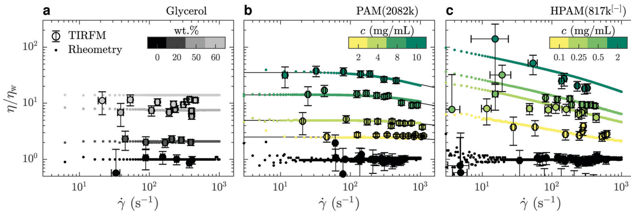
Fig. 3 Comparison of the mechanical behaviours of: (a) water/glycerol mixtures; (b) PAM(2082k) solutions; and (c) HPAM(817k l ) solutions. TIRFM velocimetry data are plotted in circles and rotational rheometry data are plotted using dots; black lines in panel (b) indicate predictions of the universal model of ref. 34. The color bars indicate the concentration of each solution and water is always represented in black. All the data shown here were collected without added salt.
