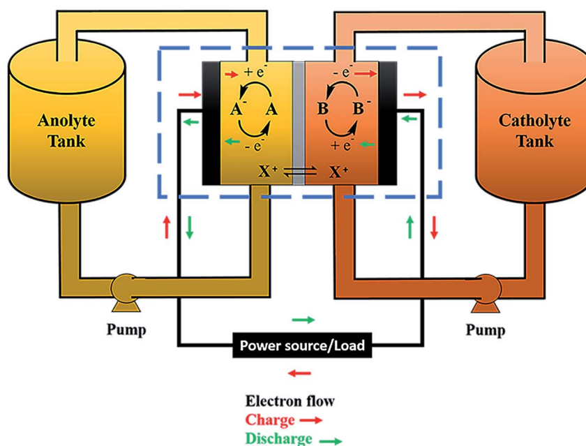
Fig. 1 General scheme of a RFB. Redox reactions take place inside the cell (marked with a blue dashed rectangle) on the surface of the electrodes (black rectangle). The electrolyte is continuously renewed by pumping the solution from the tanks. The direction of electron flow (charge or discharge) is managed by the electrical components, acting as a power source or loading the energy from the battery.
