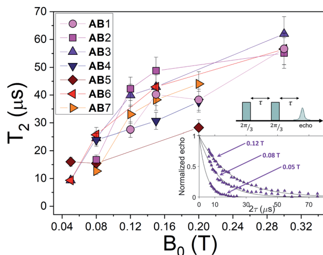
Fig. 6 Nuclear spin dephasing times T_2^{m_I, m_I'} , measured at T = 1.4 K, with the Hahn-echo sequence depicted, as a function of the applied field B_0 in the ab plane. The label of the transitions is the same reported in Fig. 4(b) and (c). Inset: Hahn echo sequence and examples of the echo decay amplitude for transition AB3 at different applied fields, fitted by an exponential function \propto e^{-2\tau/T_2} .
