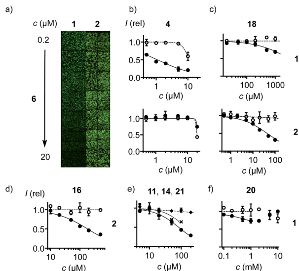
Fig. 3 (a) Fluorescence image of HCHT plates (4 images per well) with HeLa cells pre-incubated with 6 (30 min) followed by co-incubation with 1 (left) and 2 (right, 10 \mu M each) for constant 30 min. (b–f) HCHT data showing relative fluorescence intensity (filled symbols) and cell viability (empty symbols) of HeLa cells after (b) pre-incubation with 4 for 1 h, followed by washing and incubation with 1 (top), or pre-incubation with 4 for 30 min, followed by co-incubation with 4 and 2 (bottom). (c) As in (b) with 18 . (d) As in (b) after incubation for 4 h with 16 followed by incubation with 2 . (e) As in (b) after pre-incubation with 11 (circles), 14 (crosses), or 21 (diamonds) for 15 min, followed by washing and incubation with 1 . (f) As in (b) after pre-incubation with 20 (30 min), followed by washing and incubation with 1 .
