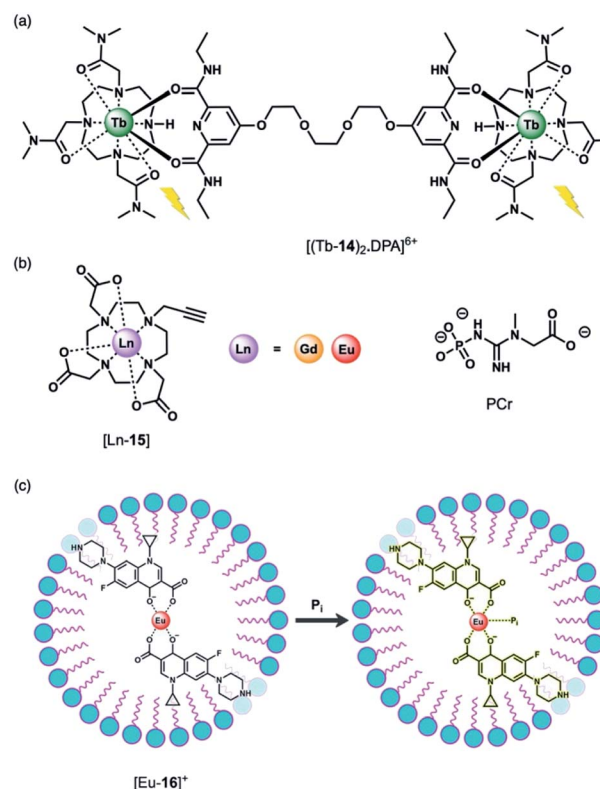
Fig. 7 (a) \text{Tb}(\text{III}) -Based displacement assay for \text{HPO}_4^{2-} and \text{NO}_3^- ; (b) alkyne-functionalised DO3A complex for assessing bulk phosphate species (PCr, \text{HPO}_4^{2-} ); (c) schematic depiction of the detection of \text{HPO}_4^{2-} ( \text{Pi} ) in water samples, using a \text{Eu}(\text{III}) -CIP mixture in the presence of the surfactant SDBS.
