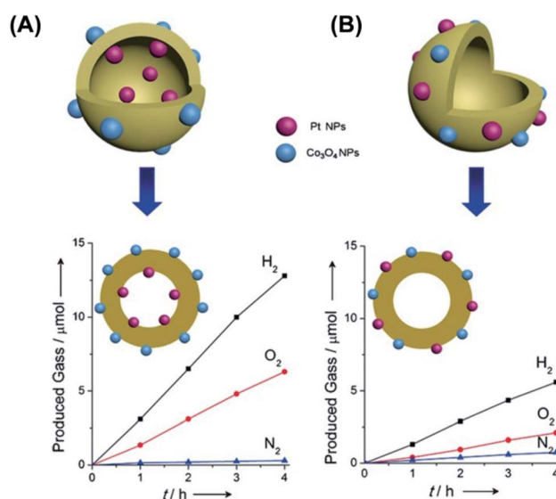
Fig. 15 Comparative results of photocatalytic water splitting under UV illumination on \text{C}_3\text{N}_4 hollow structures with (A) spatially separate co-catalysts and (B) randomly distributed co-catalysts. Reproduced with permission from ref. 138. Copyright 2016, Wiley.
