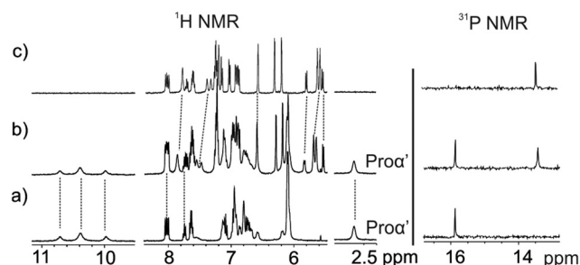
Fig. 5 ^1\text{H} NMR (400 MHz, 298 K) and ^{31}\text{P} NMR spectra of a \text{CD}_2\text{Cl}_2 solution of \text{L-ProC5in} complex before (a) and after (b) the addition of 1 equiv. of 5out . (c) ^1\text{H} and ^{31}\text{P} NMR of a \text{CD}_2\text{Cl}_2 solution of 5out .
