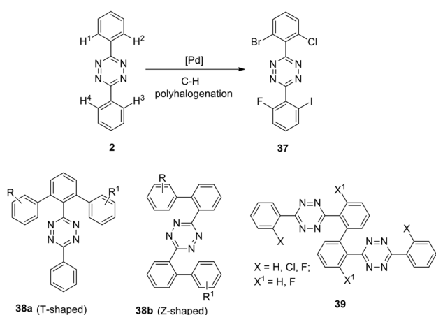
Scheme 15 The design of biphenyl tetrazines 38 with T-shaped and Z-shaped structure and bis-tetrazines 39 .
