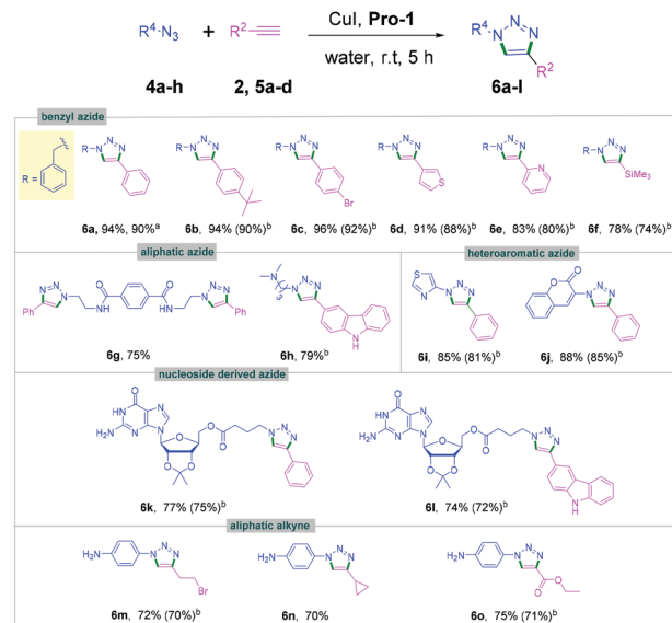
Scheme 3 Reaction of benzyl, aliphatic, heteroaromatic and nucleoside derived azides with aromatic and aliphatic alkynes, a reaction performed with 1 g of 1a for 5 h, b isolated yields after chromatographic purification.
