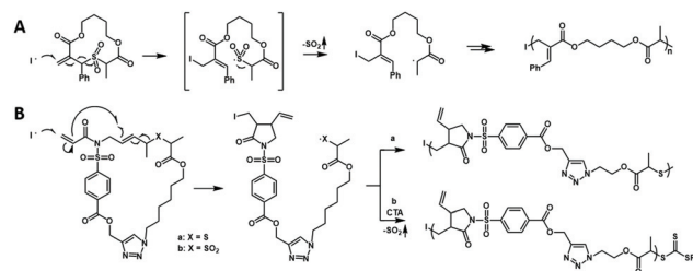
Fig. 15 (A) Radical-driven ring-opening cascade polymerization enabled by the allylic sulfone trigger. (B) Radical-driven ring-closing/cascade polymerization of macrocyclic monomers consisting of 1,6-diene-fused allylic sulfide and sulfone.
