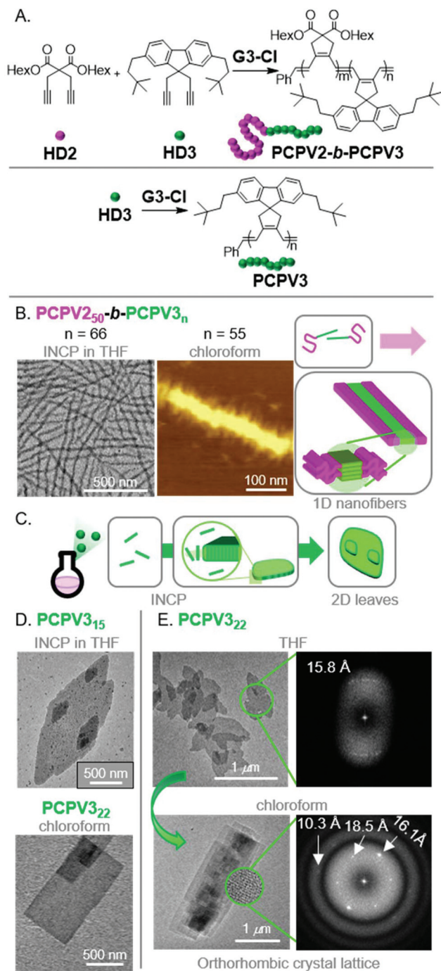
Fig. 6 (A) Synthesis of PCPV-based BCPs and homopolymers. (B) TEM (on a carbon-coated copper grid) and AFM (on mica) images of the nanofibers for \text{PCPV}_{250}\text{-}b\text{-PCPV}_{3n} . Adapted from ref. 48 with permission from the Royal Society of Chemistry, copyright 2020. (C) Proposed mechanism for 2D leaf nano-object formation via INCP. (D) TEM (on a carbon-coated copper grid) images of \text{PCPV}_{3n} -based 2D leaf nano-objects (via INCP) and rectangular nano-objects (after a non-INCP process), and (E) corresponding FFT electron diffraction patterns of each morphology. The highly ordered pattern from 2D rectangles in chloroform corresponded to the orthorhombic crystalline lattice with three main d -spacing values of 10.3, 16.1, and 18.5 Å. Adapted from ref. 49 with permission from American Chemical Society, copyright 2017.
