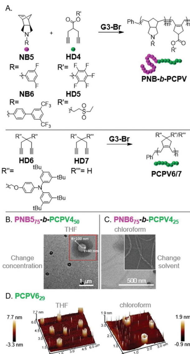
Fig. 7 (A) Synthesis of PCPV-based BCPs and homopolymers. (B) TEM (on a carbon-coated copper grid) image of \text{PNB}_{575}\text{-}b\text{-PCPV}_{450} -based vesicles formed by changing solvent concentration. Adapted from ref. 50 with permission from the Royal Society of Chemistry, copyright 2015. (C) TEM (on a carbon-coated copper grid) image of \text{PNB}_{675}\text{-}b\text{-PCPV}_{425} -based nanotubes formed by changing the dispersion solvent. Adapted from ref. 51 with permission from the Royal Society of Chemistry, copyright 2017. (D) 3D AFM (on mica) images of cylindrical nano-objects from \text{PCPV}_6 . Adapted from ref. 53 with permission from American Chemical Society, copyright 2015.
