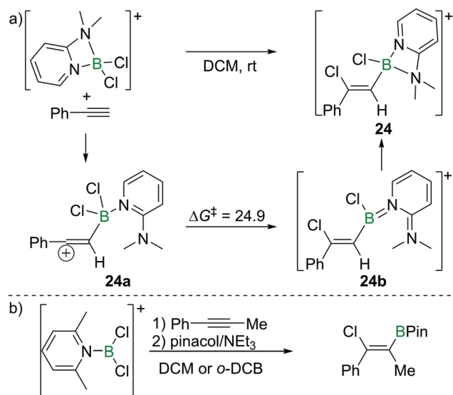
Scheme 10 Reaction route and calculated energies (kcal mol -1 ) for chloroboration of phenylacetylene with boronium/borenium complexes.
