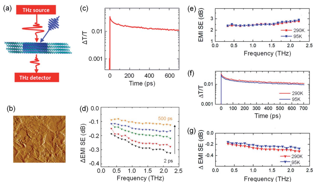
Fig. 11 (a) THz shielding modulation schematic of the MXene film stimulated by optical radiation. (b) AFM micrograph of a 25 nm-thick \text{Ti}_3\text{C}_2\text{T}_y film. (c) THz transmittance and (d) shielding effectiveness changes under different optical radiation times. (e) THz shielding effectiveness of the MXene film at 290 and 95 K without external stimuli. (f) THz transmittance changes after excitation with 800 nm and 950 \mu\text{J cm}^{-2} laser pulses at 290 and 95 K. (g) THz shielding effectiveness changes 2 ps after photoexcitation at 290 and 95 K with 800 nm and 950 \mu\text{J cm}^{-2} pulses (reproduced with permission from ref. 117 Copyright 2020 American Chemical Society).
