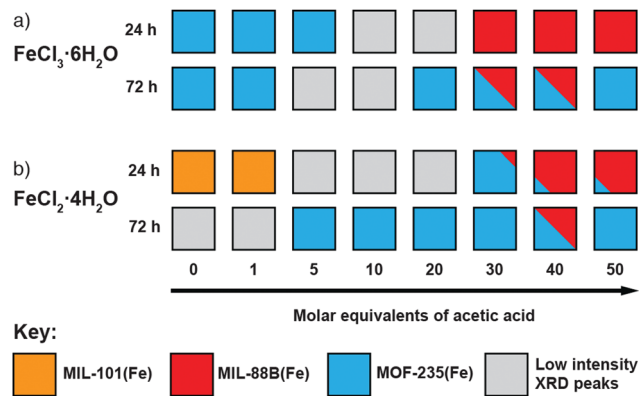
Fig. 2 Crystallisation diagrams for syntheses with (a) \text{FeCl}_3 \cdot 6\text{H}_2\text{O} and (b) \text{FeCl}_2 \cdot 4\text{H}_2\text{O} , for both 24 and 72 hours at 120 °C at each modulator concentration. Diffraction data corresponding to the figure can be found in Fig. S2, S3 (part a) and Fig. S4, S5 (part b) (ESI†).
