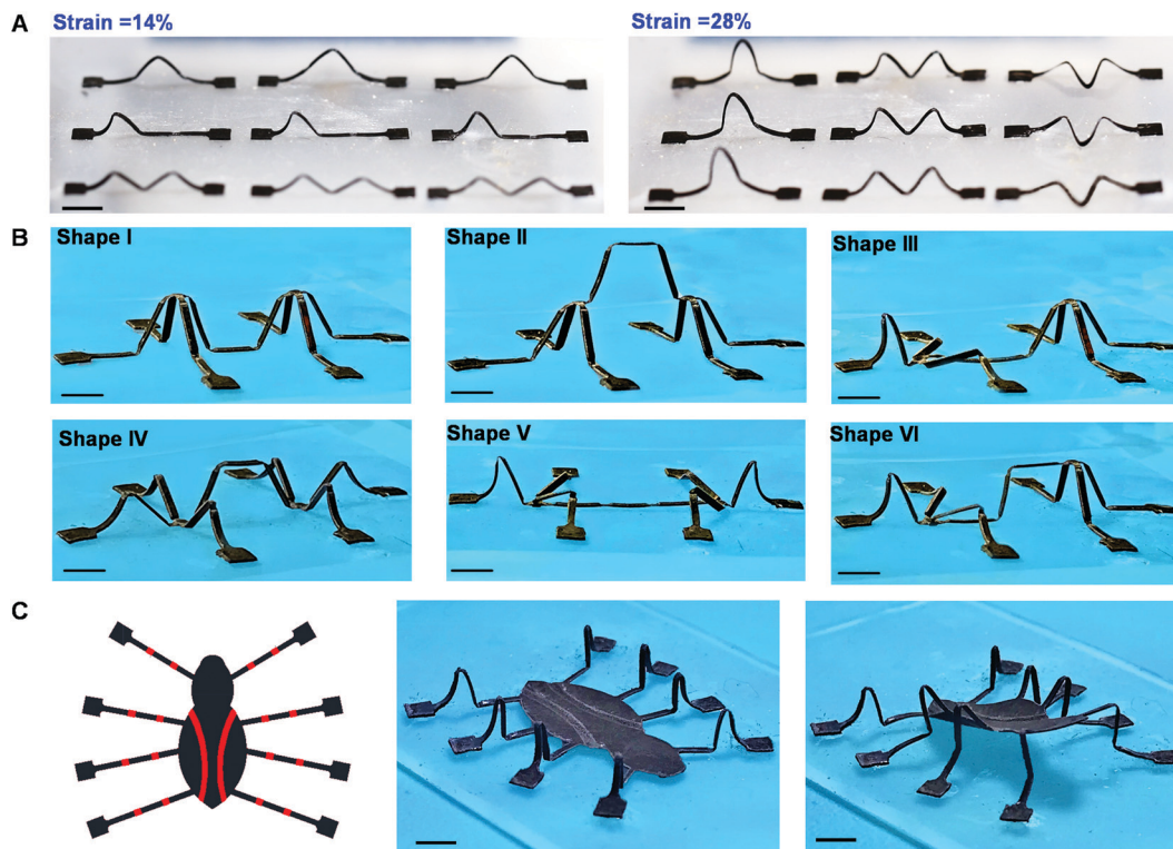
Fig. 4 Diverse origami-inspired, multistable ferromagnetic structures that can be actuated by magnetic forces. (A) An array of 3-crease ribbon structures showing different patterns formed by the multistable states of the ribbon under the strains of 14% and 28%, respectively. Scale bars, 3 mm. (B) Multistable states and magnetic reconfiguration of a double-table structure composed of creased ribbon segments. A strain of 30% is used for assembling the structure. Scale bars, 2 mm. (C) A multistable biomimetic “insect” in its flat and standing states, respectively. A strain of 30% is used for assembling the structure. Scale bars, 2 mm.
