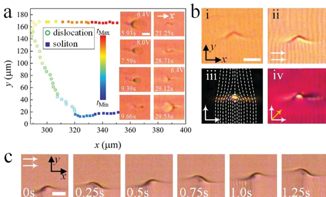
Fig. 5 Reversible transformation from a swallow-tail soliton to an edge dislocation. (a) Trajectory of a moving soliton which transforms into an edge dislocation and back to a soliton. The insets show the evolution of the transformation (scale bar 10 \mu\text{m} ). The voltage is changed between U = 6.4 V and U = 8.0 V. f = 2 Hz, T = 34.6 ^{\circ}\text{C} . (b) Optical micrographs of an edge dislocation transformed from a swallow-tail soliton (i) without polarizers, (ii) with parallel polarizers, (iii) with crossed polarizers (the white dashed lines indicate the SmA layers), (iv) with crossed polarizers and a \lambda -plate whose slow axis is orientated at 45^{\circ} to the polarizers. U = 6.6 V, f = 1 kHz, T = 34.6 ^{\circ}\text{C} , scale bar 10 \mu\text{m} . (c) Optical micrographs of an edge dislocation moving along the y -axis. U = 6.0 V, f = 2 Hz, T = 34.4 ^{\circ}\text{C} , scale bar 10 \mu\text{m} . The direction of polarizers is indicated as white arrows.
