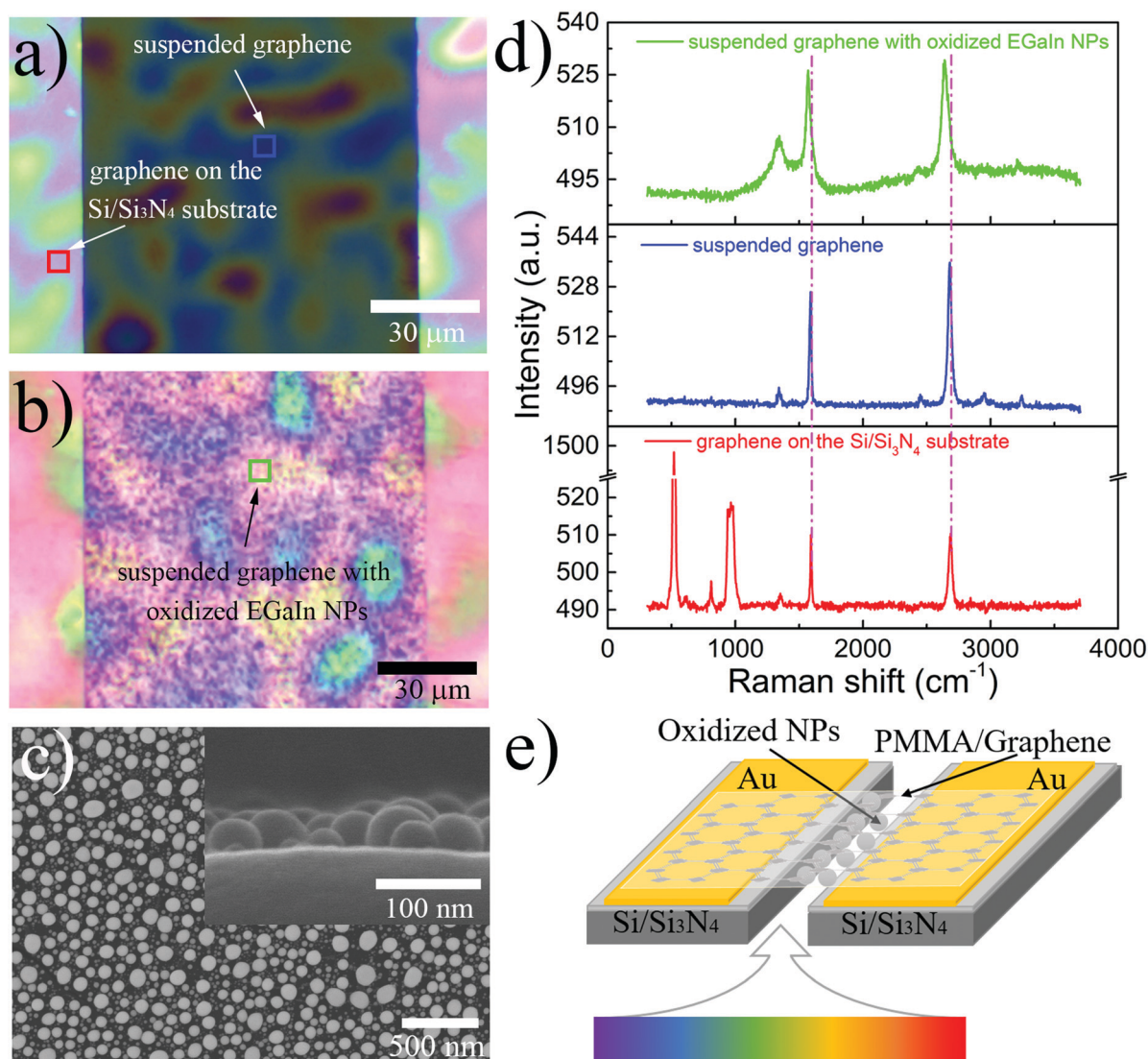
Fig. 1 Characterization of oxidized EGaIn nanoparticles on suspended graphene. (a) Microscope images of few-layer graphene suspended on Si/Si 3 N 4 substrate with a 100 μm-wide slit. (b) Microscope image of suspended graphene composited with oxidized EGaIn nanoparticles. The 5\ \mu\text{m} \times 5\ \mu\text{m} squares in the (a) and (b) are the measuring location for the Raman spectra. (c) The SEM image of oxidized EGaIn nanoparticles on the suspended graphene. The inset shows cross-section SEM images of EGaIn on the graphene. (d) The Raman spectra for graphene on the Si/Si 3 N 4 substrate, suspended graphene and suspended graphene with oxidized EGaIn nanoparticles. (e) Schematic of the device structure. The laser can illuminate the composite part through the slit from the bottom.
