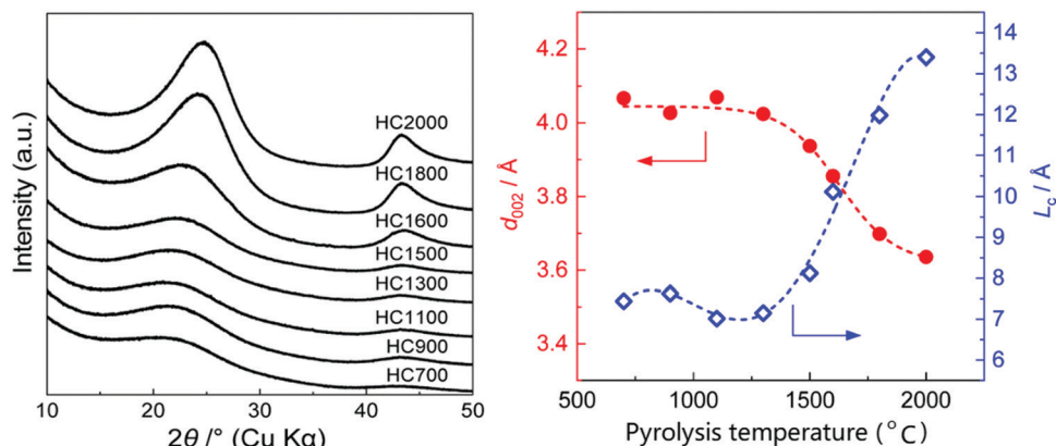
Fig. 18 (a) XRD patterns of sucrose-derived HC samples pyrolysed at temperatures between 700 and 2000 ^{\circ}\text{C} , and (b) relationship between d -spacing and graphitic crystallite length along the c -axis as a function of pyrolysis temperature. 84 Copyright 2020, American Chemical Society.
