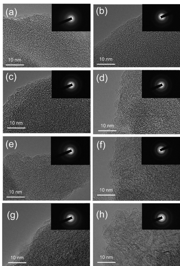
Fig. 19 TEM images showing the crystallite size of sucrose-derived HC samples pyrolysed at (a) 700, (b) 900, (c) 1100, (d) 1300, (e) 1500, (f) 1600, (g) 1800, and (h) 2000 ^{\circ}\text{C} . 84 Copyright 2020, American Chemical Society.
