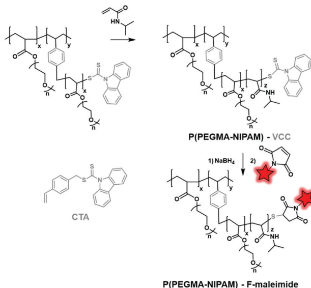
Fig. 33 CTA reduction by \text{NaBH}_4 , followed by fluorescent labeling as described by Feijen et al.
