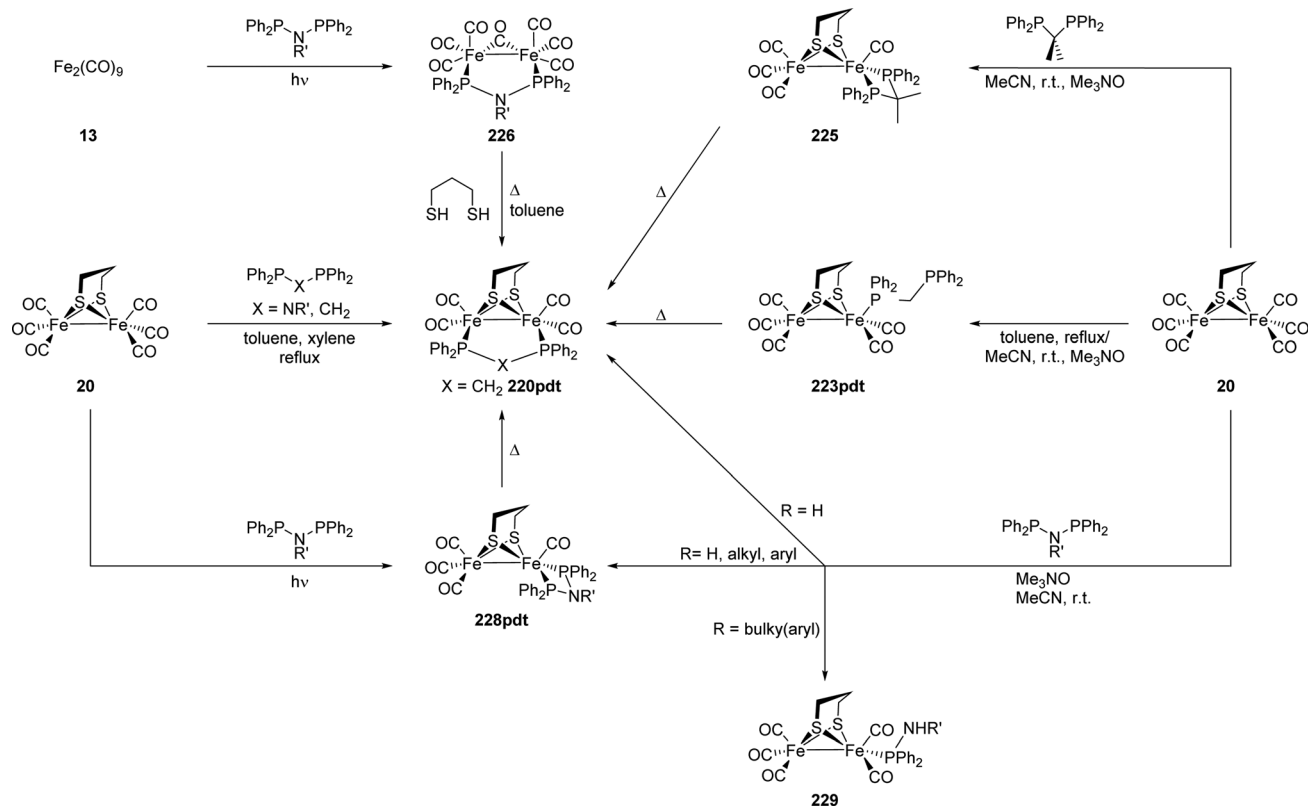
Fig. 65 Different synthetic pathways for the incorporation of dpmp and derived ligands as well as PNP ligands into hydrogenase mimics.
