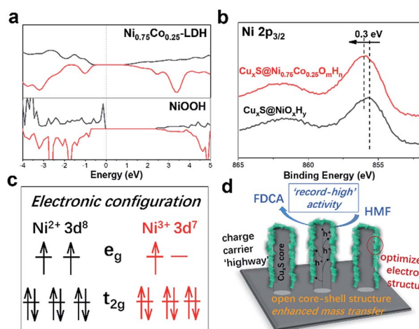
Fig. 4 (a) Projected density of states calculations for \text{Ni}_{0.75}\text{Co}_{0.25}\text{-LDH} and NiOOH. (b) High resolution Ni 2p 3/2 XPS spectra of \text{Cu}_x\text{S}@ \text{Ni}_{0.75}\text{Co}_{0.25}\text{O}_m\text{H}_n and \text{Cu}_x\text{S}@ \text{NiO}_m\text{H}_n . (c) Schematic illustration of the electronic configuration of the Ni cations with valence states of +2 and +3. (d) Schematic illustration of factors contributing to the high HMF oxidation activity.
