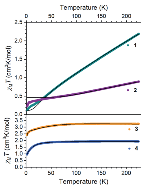
Fig. 4 Dc magnetic susceptibility data for 1–4 collected under an applied magnetic field of 1000 Oe. Black lines represent fits to the data.
