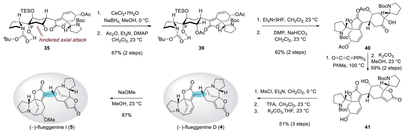
Scheme 5 Total synthesis of (-)-flueggegenines D (4) and I (5).
