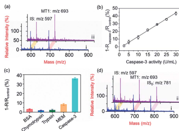
Fig. 2 Quantification of caspase-3 activity. (a) MALDI mass spectra of the PRMNTs-Casp-3 incubated with 25 \text{U mL}^{-1} caspase-3 (i) or the blank solution (ii) at 37 ^{\circ}\text{C} for 1.5 h. (b) The linear correlation between the relative variation of the intensity ratio and caspase-3 activity. The peak intensity ratio of MT1 to IS of the PRMNTs-Casp-3 incubated with caspase-3 was denoted as R_{\text{caspase-3}} , and that incubated with the blank solution was denoted as R_{\text{control}} . (c) The relative variation of the intensity ratio ( 1 - R/R_{\text{control}} ) in PRMNTs-Casp-3 after incubation with 25 \text{U mL}^{-1} caspase-3 for 1.5 h or 4 mM GSH, 50 \mu\text{g mL}^{-1} BSA, 10 \mu\text{g mL}^{-1} chymotrypsin, 10 \mu\text{g mL}^{-1} trypsin or MEM buffer for 12 h. (d) MALDI mass spectra of the PRMNTs-Casp-3 with (i) or without (ii) incubation of 4 mM GSH at 37 ^{\circ}\text{C} for 12 h. Just before the sample loading for MALDI MS analysis, AuNPs@MT2 (ion signal denoted as \text{IS}_0 ) were added as the reference to assess the relative ion signals of MT1 and IS.
