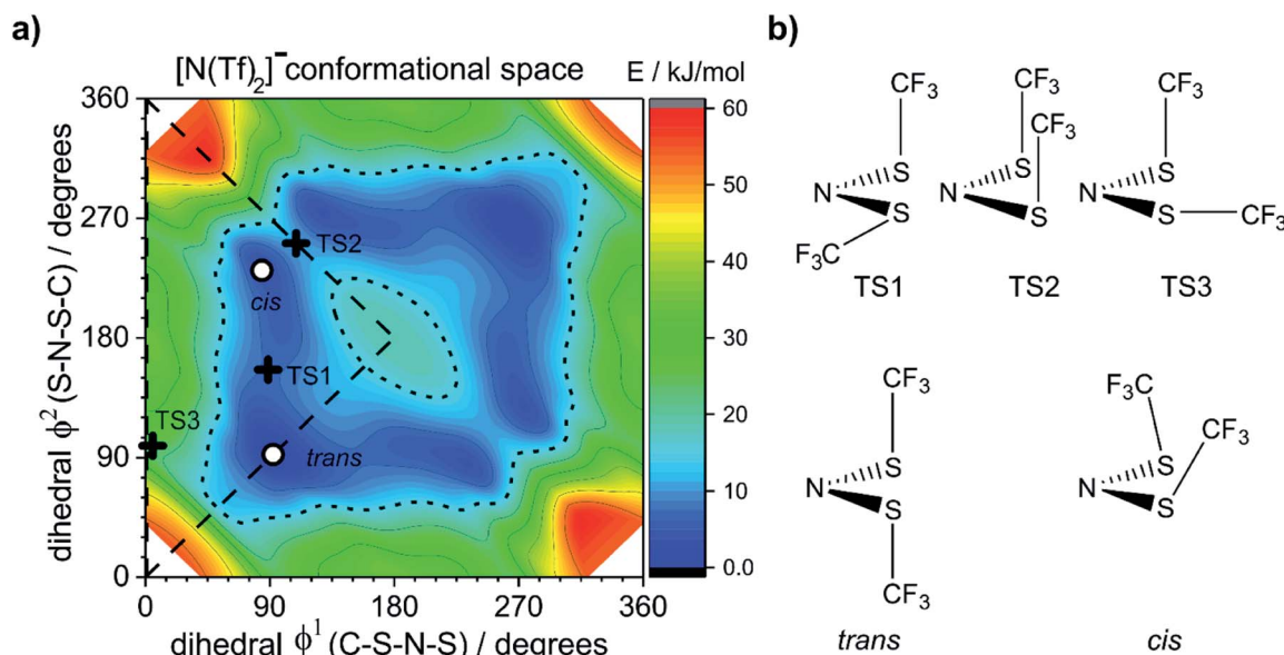
Fig. 5 (a) PES of [N(Tf)_2]^- , (b) stationary point structures (oxygen atoms not shown). Open circles denote minima, black crosses denote transition states. The dotted line is drawn at 15 \text{ kJ mol}^{-1} to facilitate comparison with other surfaces. The lowest energy conformer is taken as the zero reference.
