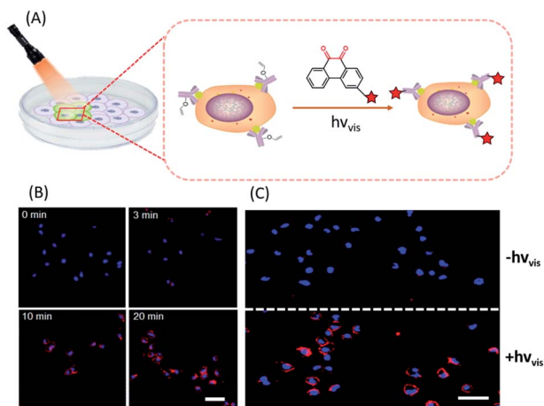
Fig. 5 Spatiotemporal labelling of live cells realized by the visible-light driven DVPC reaction (scale bar: 50 \mu m).
