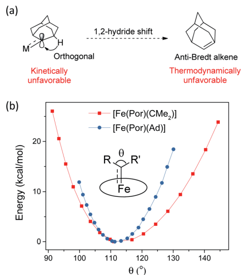
Fig. 15 (a) Resistance of \text{M}\equiv\text{Ad} complexes toward 1,2-hydride shift. (b) Calculated potential energy curves for [\text{Fe}(\text{Por})(\text{Ad})] and [\text{Fe}(\text{Por})(\text{CMe}_2)] by changing the angle \theta .
