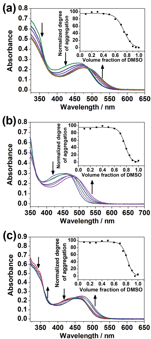
Fig. 5 UV-Vis absorption spectra of (a) 5, (b) 6 and (c) 7 in DMSO ([Pt] = 4.0 \times 10^{-5} M) with increasing water content (a) from 20 to 90%, (b) from 10 to 40% and (c) 5 to 30%. Insets: plots of normalized degree of aggregation of the complexes against volume fraction of DMSO.
