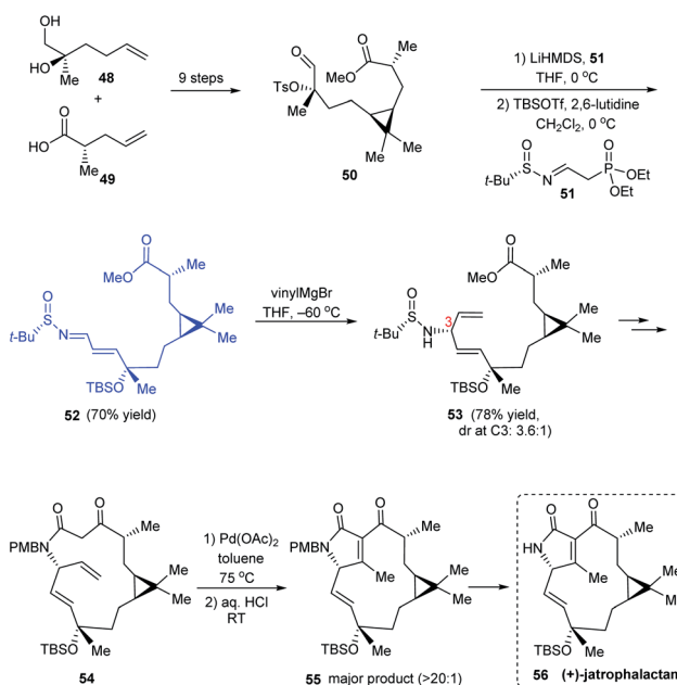
Scheme 11 Synthesis of (+)-jatrophalactam 56 .
