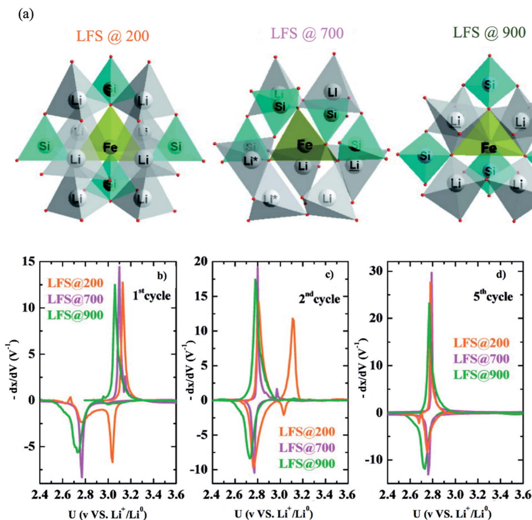
Fig. 15 (a) The three polymorphs of \text{Li}_2\text{FeSiO}_4 , derivative plots obtained from PITT measurements in the (b) first, (c) second, and (d) fifth cycles for all three polymorphs. 141
