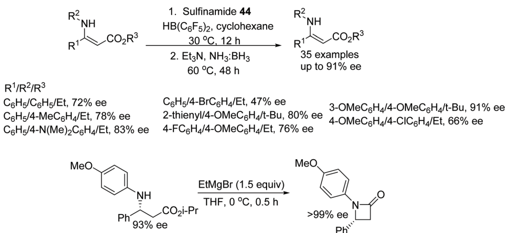
Fig. 58 CPA catalysed ATH of \beta -N-substituted enamine esters and construction of chiral \beta -lactam.
