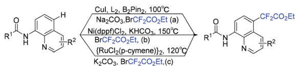
Scheme 89 The Cu-, Ni-, Ru-catalyzed difluoroalkylation of 8-aminoquinolines.
