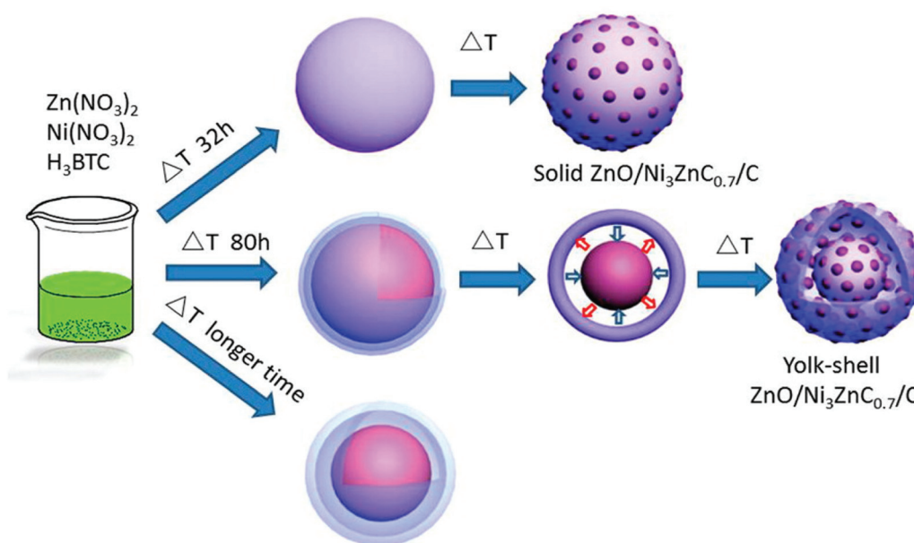
Fig. 4 Preparation process of yolk-shell \text{ZnO}/\text{Ni}_3\text{Zn}_{0.7}\text{C}/\text{C} . 48
