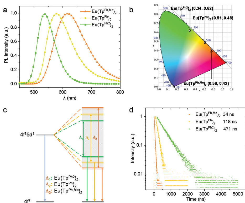
Fig. 2 (a) Solid steady-state PL spectra (photoexcitation wavelength: 365 nm) of \text{Eu}(\text{Tp}^{\text{Ph,Me}})_2 , \text{Eu}(\text{Tp}^{\text{Ph}})_2 and \text{Eu}(\text{Tp}^{\text{Ph2}})_2 . (b) The CIE 1931 chromaticity diagram of \text{Eu}(\text{Tp}^{\text{Ph,Me}})_2 , \text{Eu}(\text{Tp}^{\text{Ph}})_2 and \text{Eu}(\text{Tp}^{\text{Ph2}})_2 . (c) Orbital-energy diagram for the ligand field splitting of the d orbitals (double arrow) and the energy transition (single arrow) of \text{Eu}(\text{Tp}^{\text{Ph,Me}})_2 , \text{Eu}(\text{Tp}^{\text{Ph}})_2 and \text{Eu}(\text{Tp}^{\text{Ph2}})_2 . (d) Transient PL spectra of \text{Eu}(\text{Tp}^{\text{Ph,Me}})_2 , \text{Eu}(\text{Tp}^{\text{Ph}})_2 and \text{Eu}(\text{Tp}^{\text{Ph2}})_2 .
