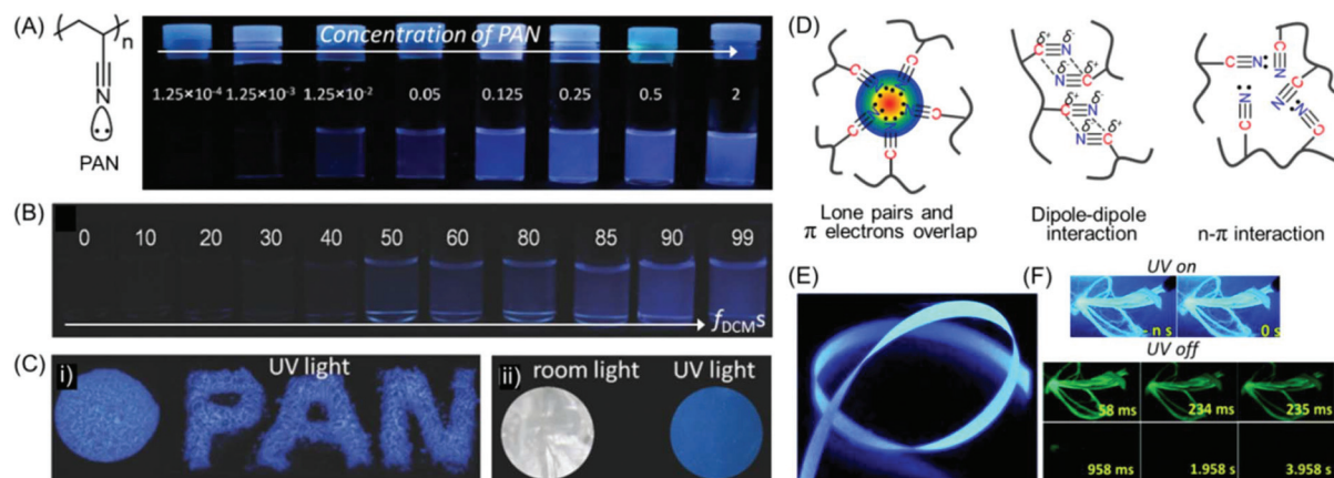
Fig. 8 (A) Chemical structure of intrinsically emissive PAN. Photographs of PAN in only DMF and (B) a DCM/DMF mixture with various f_{\text{DCM}} s obtained under a 365 nm UV lamp. (C) Luminescence images of (i) solid powders and (ii) a film of PAN on exposure to 365 nm UV excitation. (D) Schematic illustration of plausible intra- and inter-molecular interactions present within nitrile clusters in the aggregated state. (E) Photoluminescence image of SR6 ENRs taken under 365 nm UV irradiation. (F) Photographic images of ENRs at 77 K in UV lamp-on/lamp-off mode at different time courses. Figures A, B, C and D are reprinted with permission from ref. 55. Copyright (2016), John Wiley and Sons. Figures E and F are reprinted with permission from ref. 57. Copyright (2020), Royal Society of Chemistry.
