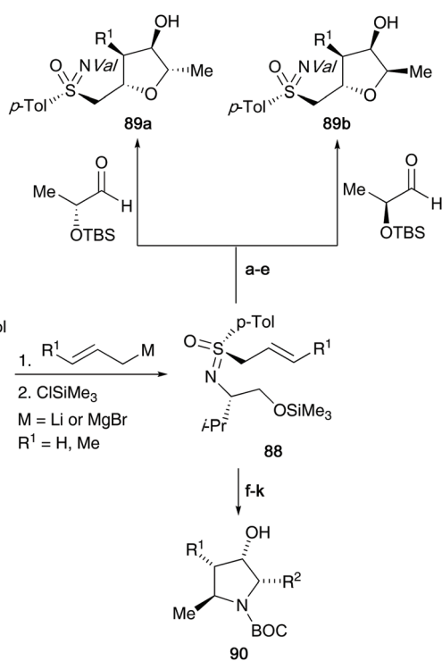
Scheme 23 Application of 2-alkenylsulfoximines 88 towards the construction of important organic heterocycles 89 and 90 . Reaction conditions: (a) n\text{BuLi} , THF, -78^\circ\text{C} ; (b) \text{ClTi}(\text{O}i\text{Pr})_3 , 0^\circ\text{C} ; (c) aldehyde, -78^\circ\text{C} ; (d) (\text{NH}_4)_2\text{CO}_3 ; (e) \text{Bu}_4\text{NF} ; (f) n\text{-BuLi} , toluene, -78^\circ\text{C} ; (g) \text{ClTi}(\text{O}i\text{Pr})_3 , 0^\circ\text{C} ; (h) Fmoc-protected \alpha -aminoaldehydes, -78^\circ\text{C} ; (i) piperidine, 20^\circ\text{C} , (\text{NH}_4)_2\text{CO}_3 , \text{NH}_4\text{Cl} ; (j) \text{K}_2\text{CO}_3 , MeOH; \text{BOC}_2\text{O} , \text{NaHCO}_3 ; (k) \text{Sml}_2 .
