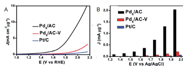
Fig. 5 (A) OER polarization curves. (B) Mass OER activity of Pd 6 /AC, Pd 6 /AC-V and Pt/C at each overpotential. Panels (a) and (b) are reproduced with permission from ref. 26. Copyright 2017 Royal Society of Chemistry.
