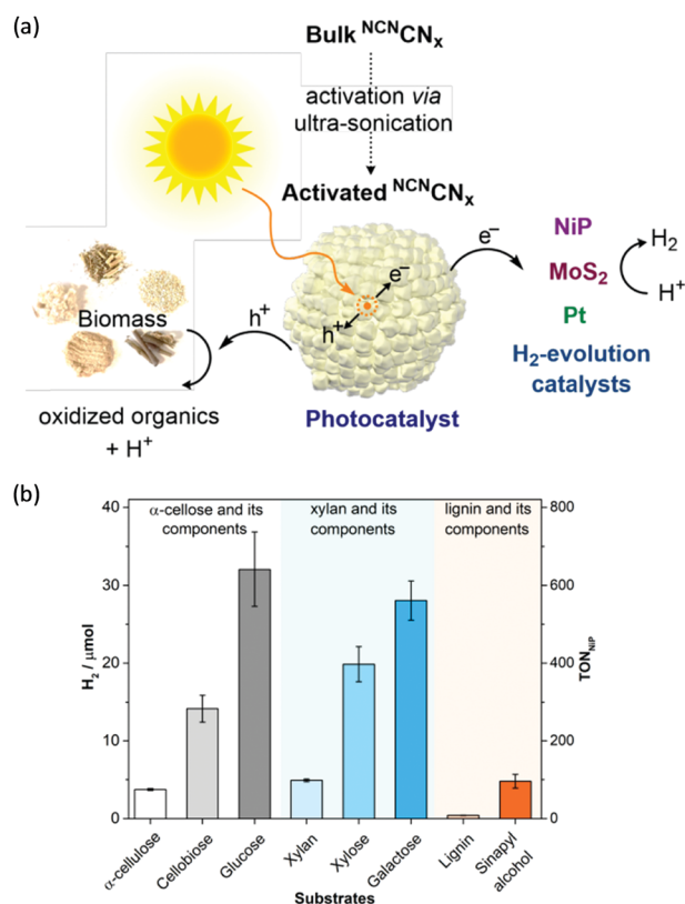
Fig. 6 (a) Schematic photo-reforming of lignocellulose using NCN CN x and proton reduction co-catalysts. (b) Photocatalytic H 2 production from purified lignocellulose components catalyzed by activated NCN CN x and NiP under AM1.5G light irradiation for one day at 25 °C. Reprinted from ref. 48 with permission of American Chemical Society, copyright 2018.
