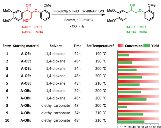
Fig. 6 Catalytic dehydrogenative decarbonylation A-OEt or A-OBu to B-OEt or B-OBu. Reaction conditions: 15 mg substrate, [\text{Ir}(\text{cod})\text{Cl}]_2 5 mol%, 4 : 2 : 1 LiCl : rac -BINAP : [\text{Ir}(\text{cod})\text{Cl}]_2 , as catalyst; 190–210 °C in 1 mL solvent. Yield and conversion were determined by GC-FID using n -decane as an external standard; *Set temperature of the heating block; the measured corresponding inside temperature is shown in Table S1.†
