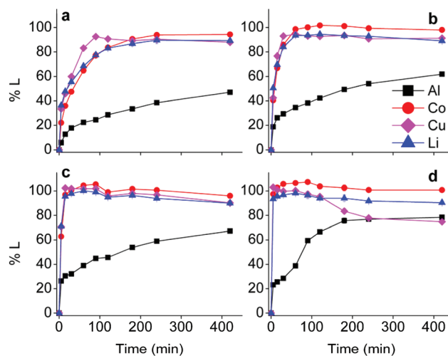
Fig. 1 Leaching efficiencies (%L) of \text{LiCoO}_2 + Al + Cu mixtures in choline chloride–citric acid DES as a function of time at different temperatures. Temperatures: room temperature (left above, a), 40 °C (right above, b), 60 °C (left below, c) and 80 °C (right below, d). DES: ChCl : CA 2 : 1 + 35 wt% H 2 O. Leaching parameters: S : L = 20 g L -1 , Al : \text{LiCoO}_2 = 12 wt%, Cu : \text{LiCoO}_2 = 24 wt% at 900 rpm.
