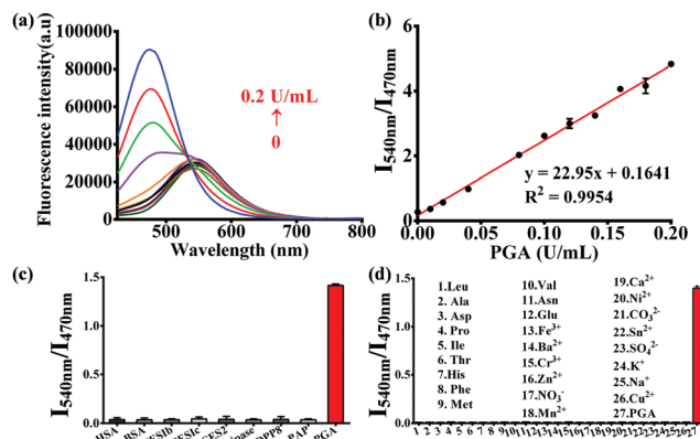
Fig. 1 (a) Fluorescence spectra of PNA (10 \mu M) upon addition of increasing concentrations of PGA (0–0.2 U mL -1 ). (b) Linear relationship between the fluorescence ratio ( I_{540}/I_{470} ) and PGA concentration. Fluorescence intensity ratio ( I_{540}/I_{470} ) of PNA upon addition of various enzymes and proteins (c), ions and amino acids (d). (PGA 0.05 U mL -1 , PBS : acetonitrile 2 : 1, v/v, \lambda_{\text{ex}} 400 nm).
