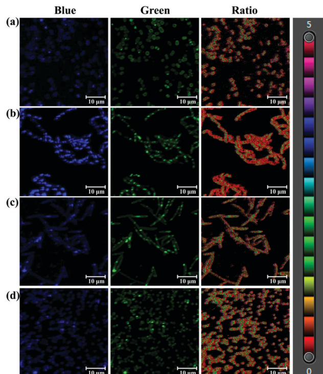
Fig. 2 Fluorescence images of bacteria incubated with PNA (50 \mu M). (a) Acinetobacter baumannii LMG 994 HAM (ratio 1.995). (b) Bacillus cereus 994000168 LBK (ratio 0.41). (c) Brevibacillus parabrevis 090915_03 LBK (ratio 1.135). (d) Staphylococcus aureus ssp. aureus DSM 799 DSM (ratio 0.842). Blue channel: \lambda_{\text{ex}} 405/ \lambda_{\text{em}} 425–459 nm, green channel: \lambda_{\text{ex}} 405/ \lambda_{\text{em}} 525–575 nm. Scale bar 10 \mu m.
