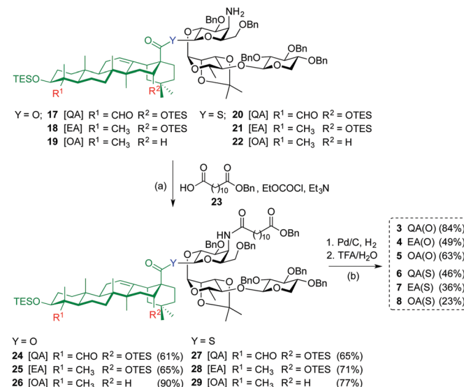
Scheme 2 Reagent and conditions: (a) \text{EtOCOCl} , \text{Et}_3\text{N} , THF, 0 °C to r.t., 4 h, 61% (for 24 ), 65% (for 25 ), 90% (for 26 ); 65% (for 27 ), 71% (for 28 ), and 77% (for 29 ); (b) 1: Pd/C, \text{H}_2 (1 atm), \text{EtOH}/\text{THF} 1 : 1, r.t., 16 h (for 24–26 ); 20 min (for 27–29 ); 2: TFA/ \text{H}_2\text{O} 3 : 1, 0 °C, 1 h, 84% (for 3 ), 49% (for 4 ), 63% (for 5 ); 46% (for 6 ), 36% (for 7 ), and 23% (for 8 ).
