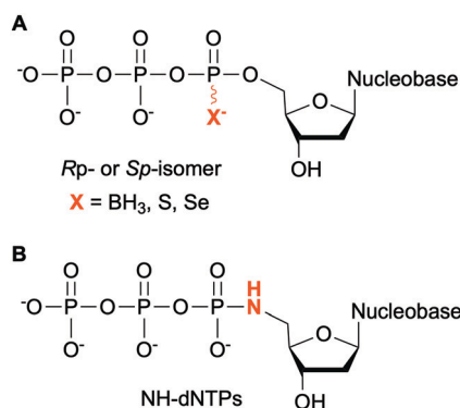
Fig. 9 Modifications at the \alpha -phosphate of non-natural NTPs.
