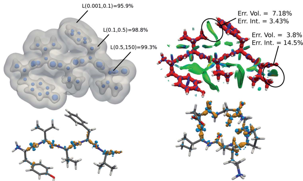
Fig. 7 (top left) predicted electron density of enkephalin (PDB ID: 4OLR) at three isovalues: 0.5, 0.1, and 0.001 \text{e}^- \text{bohr}^{-3} . For each isosurface, the L(a,a') similarity index with respect to ab initio density is reported. (top right) DORI map of enkephalin (DORI isovalue: 0.9) colored by \text{sgn}(\lambda_2)\rho(r) in the range from -0.02 a.u. (red) to 0.02 a.u. (blue) (lower left) density difference between predicted and ab initio electron density (isovalues \pm 0.01 \text{e}^- \text{bohr}^{-3} ). (lower right) density difference between predicted and ab initio electron density of 3WNE (isovalues \pm 0.01 \text{e}^- \text{bohr}^{-3} ).
