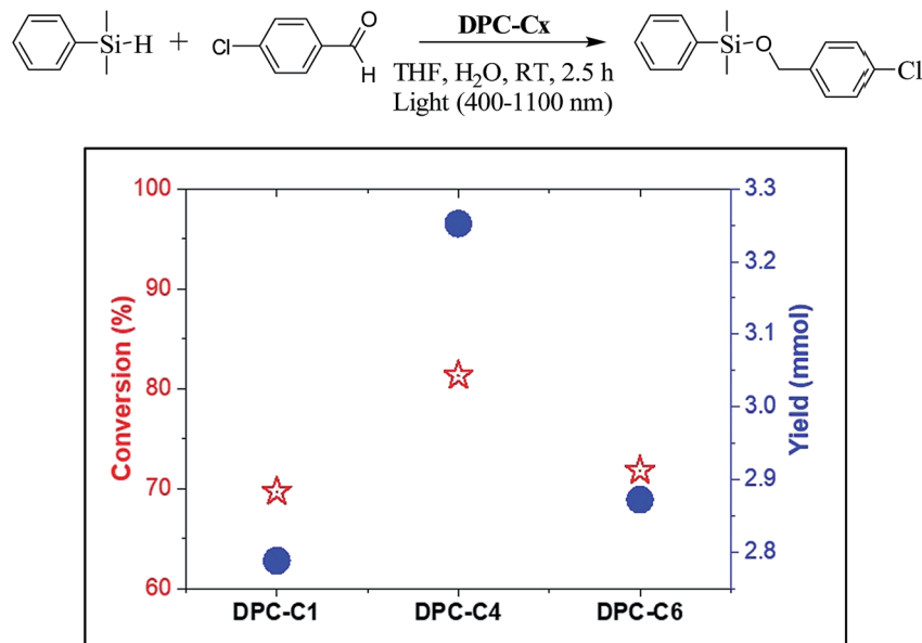
Fig. 13 Conversion and product yield for hydrosilylation of aldehydes using DPC-C1, DPC-C4, and DPC-C6 as catalysts at 25 °C using 400–1100 nm light in 2.5 h.
